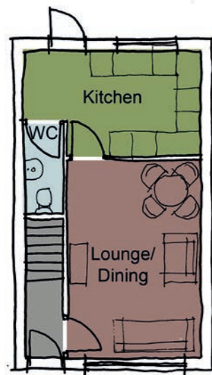
TYPICAL HOUSE PLANS - 2 BED (67.5 SQM) - 2 STOREY HOUSE
